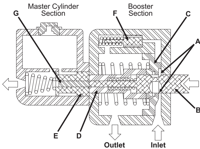
Figure 6 Two Fluid Power Brake Actuator
