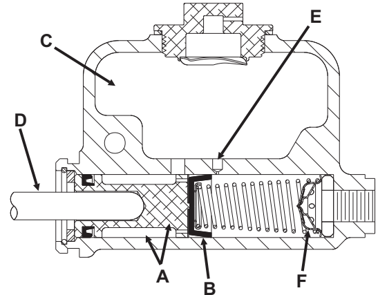
Figure 1 Straight Bore Master Cylinder
