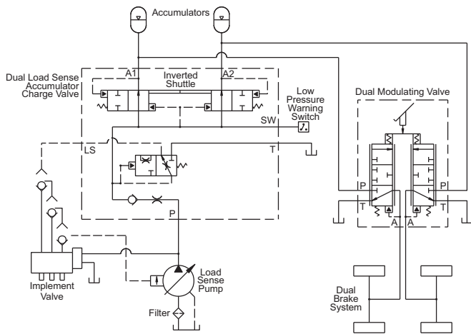
Figure 13 Dual Closed Center Brake Circuit in a Non-Dedicated Load Sense Hydraulic System
