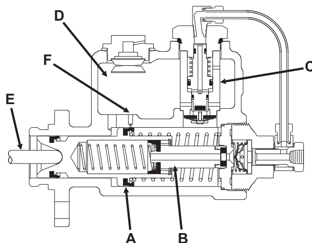
Figure 3 Power Cylinder
