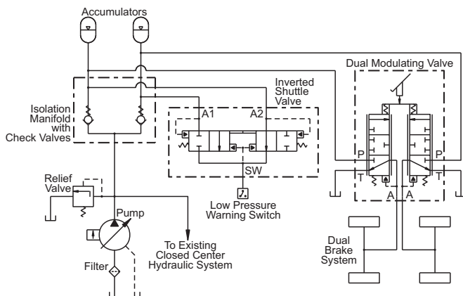
Figure 14 Dual Closed Center Brake Circuit in a Non-Dedicated Closed Center Hydraulic System
