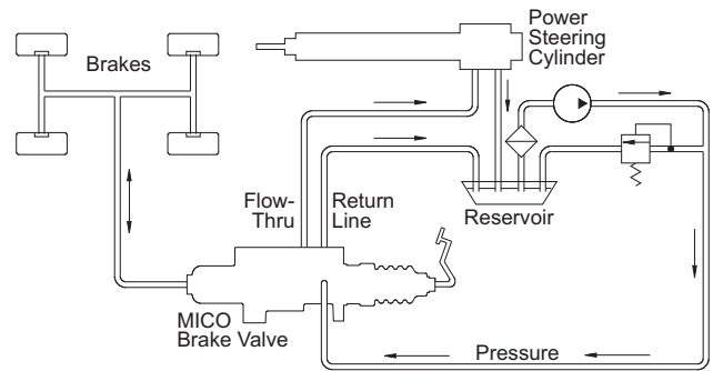
Figure 4 Open Center Power Brake System Typical Circuit
