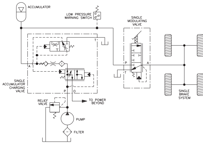
Figure 11 Single Closed Center Brake Circuit in a Non-Dedicated Open Center Hydraulic System
