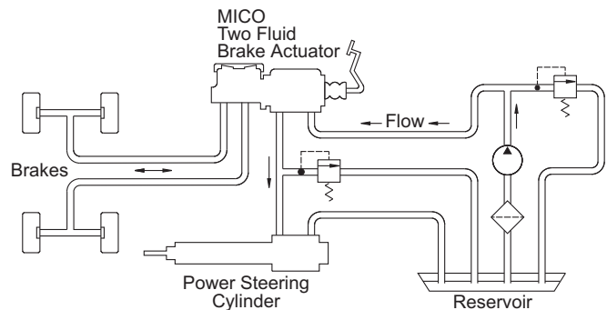
Figure 8 Open Center Two Fluid Hydraulic Brake System Typical Circuit
