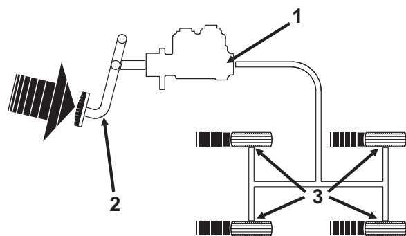
Figure 2 Simple Non-Boosted Brake System
