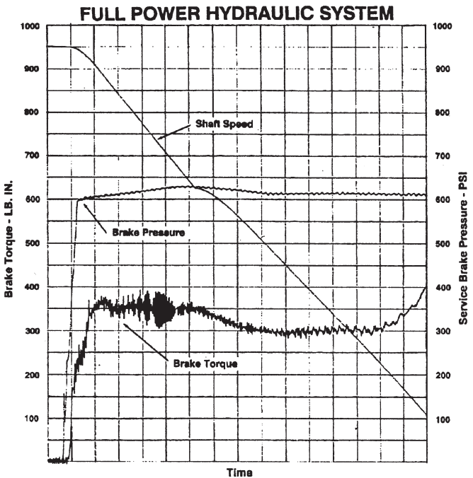
Figure 10 Time response - Full Power hydraulic
