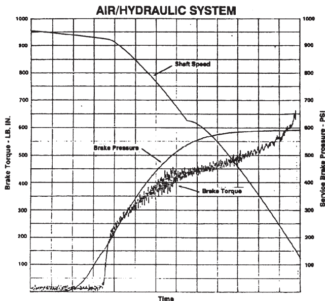
Figure 9 Time response - Air/hydraulic
