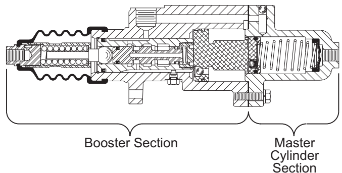
Figure 5 Open Center Power Brake Valve
