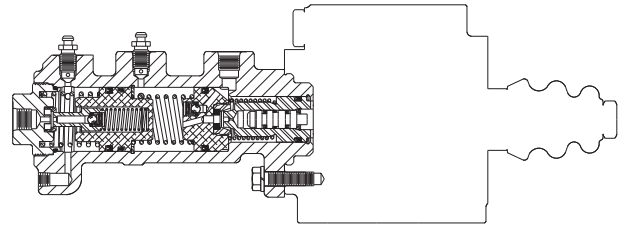
Figure 7 Two Fluid Tandem Master Cylinder
