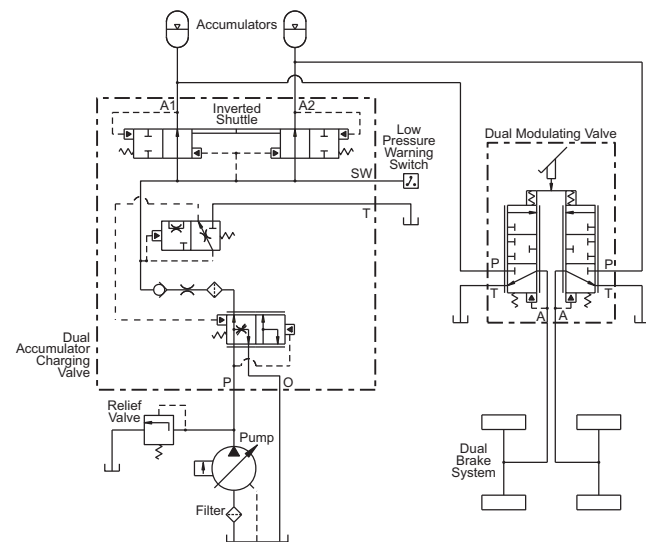
Figure 12 Dual Closed Center Brake Circuit in a Dedicated Open Center Hydraulic System
