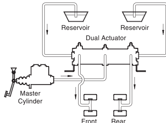
Single system split
