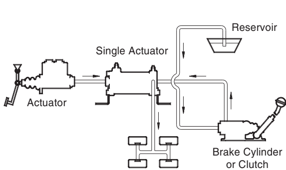
Actuator override for two remote positions
