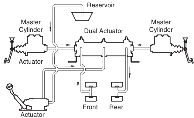
Three position actuator override
