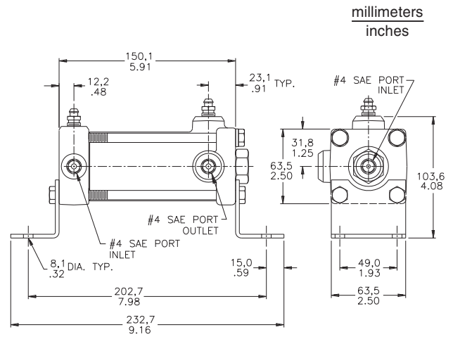
Single Actuator (1 3/4 inch diameter bore)
