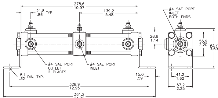
Dual Actuator (1 1/4 inch diameter bore)
