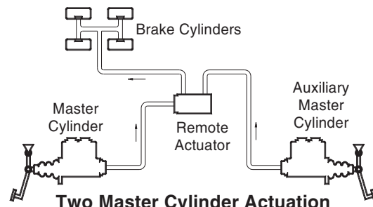
Two Master Cylinder Actuation
