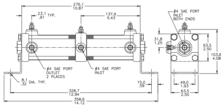
Dual Actuator (1 3/4 inch diameter bore)
