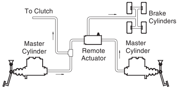
Two Master Cylinder Actuation
