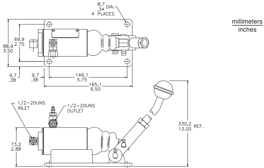
Non-ratchet lever type handle
