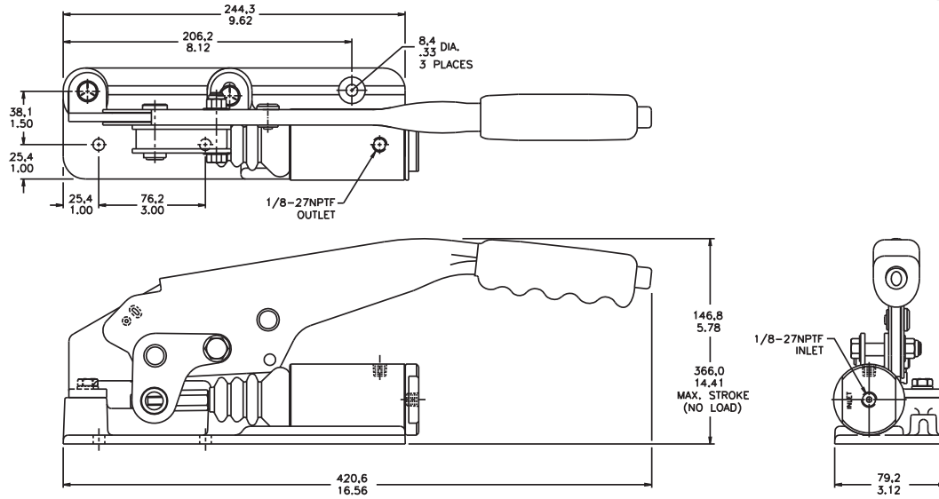
Ratchet lever type handle
