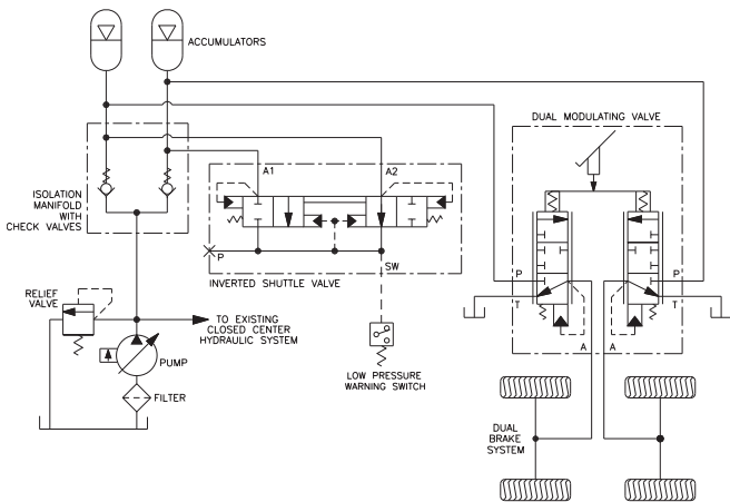
Figure 14 Dual Closed Center Brake Circuit in a Non-Dedicated Closed Center Hydraulic System
