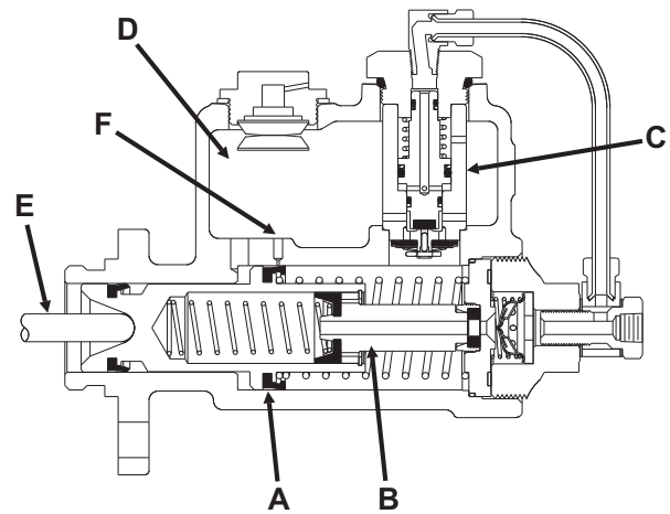
Figure 3 Power Cylinder
