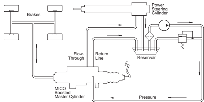
Figure 4 Open Center Power Brake System Typical Circuit
