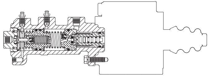
Figure 7 Two Fluid Tandem Master Cylinder
