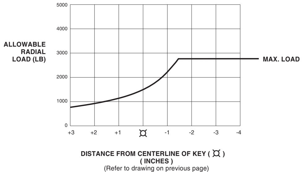
LOAD CAPACITY @ 240 RPM AND B 10 = 3000 HRS
